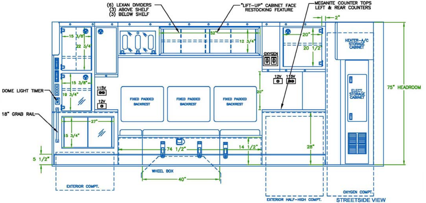
Streetside Layout
