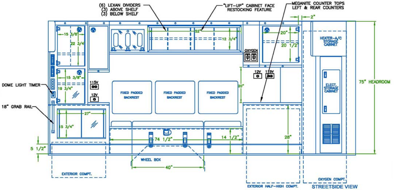
Streetside Layout
