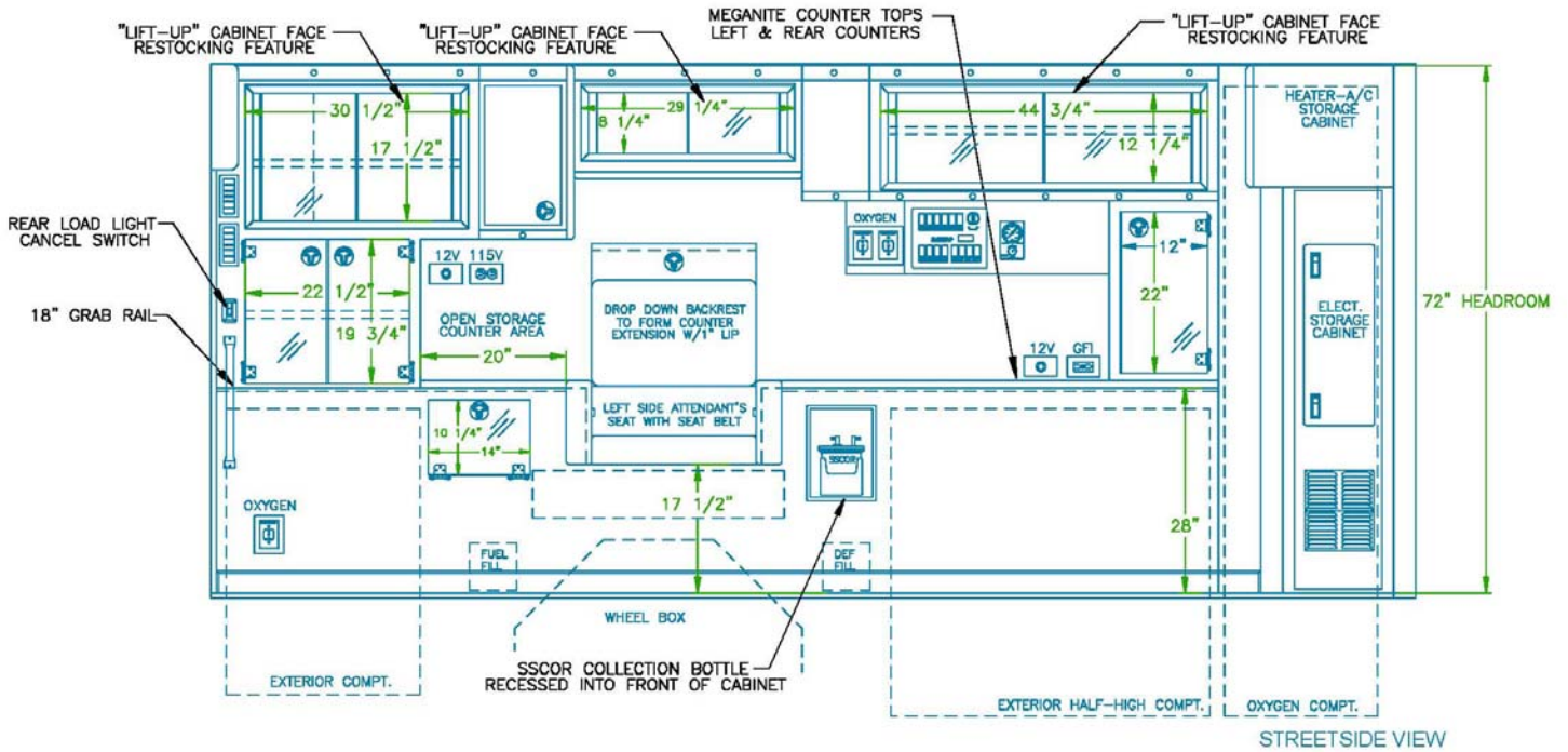
Streetside Layout
