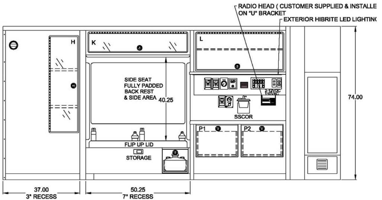
Streetside Layout
